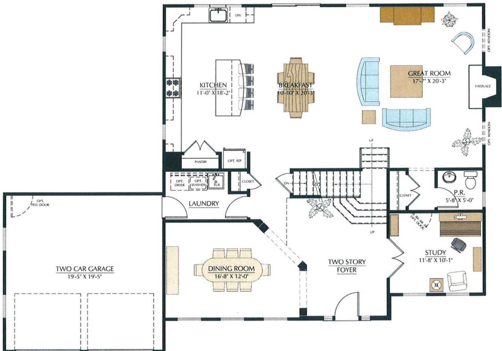
FIRST FLOOR WITH STANDARD KITCHEN LAYOUT
